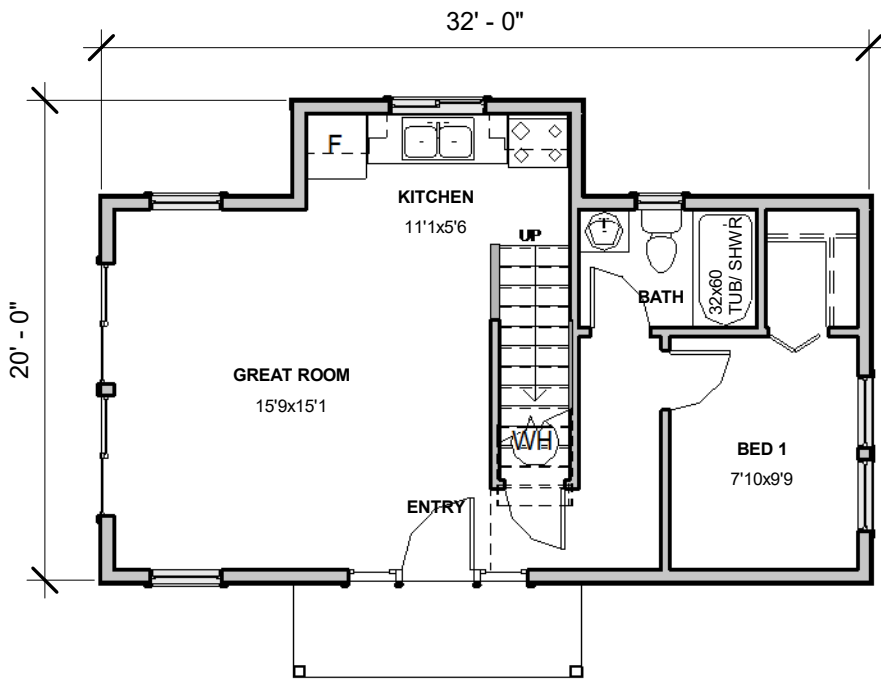
MAIN FLOOR - 560sf
