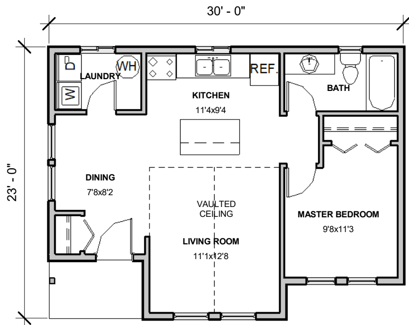
MAIN FLOOR - 1 Bedroom Option
