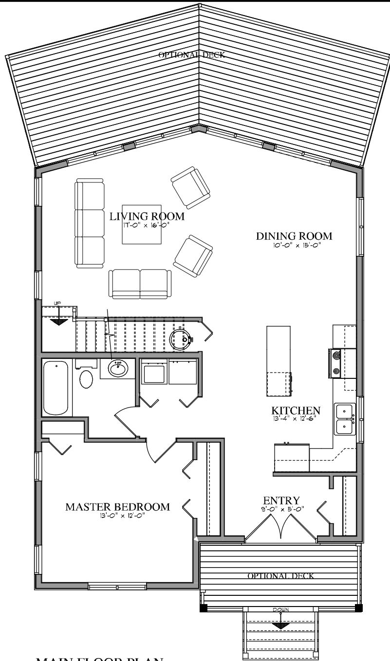
MAIN FLOOR PLAN 1000 SF
